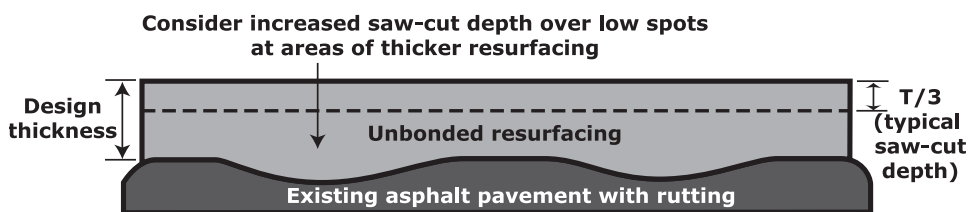
Figure 6. Consider asphalt rut depth when determining saw-cut depth (ACPA 1998)
